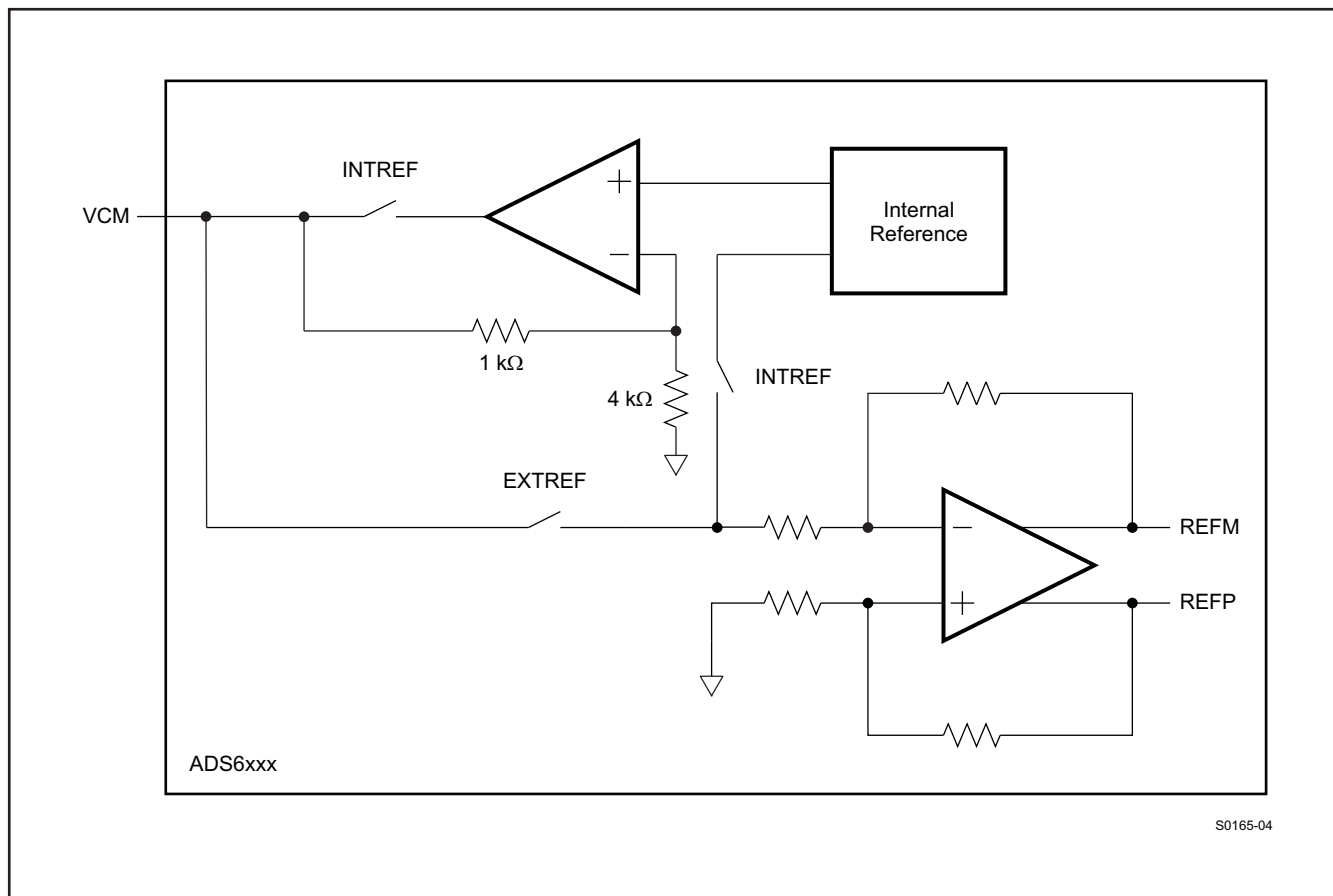
Figure 88. Reference Section
