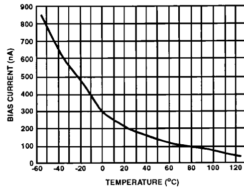
FIGURE 11. BIAS CURRENT vs TEMPERATURE
