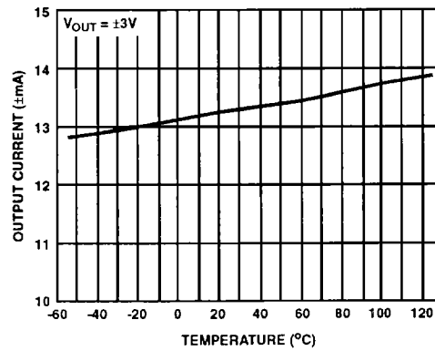
FIGURE 15. OUTPUT CURRENT vs TEMPERATURE
