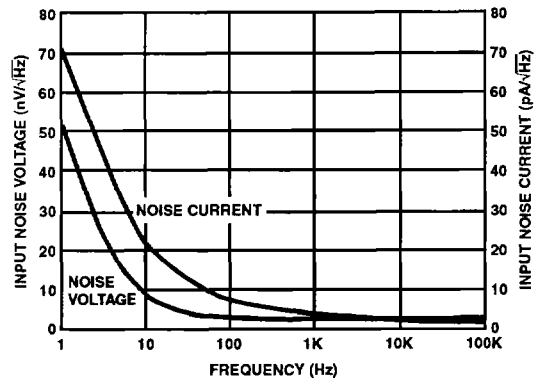
FIGURE 25. INPUT NOISE vs FREQUENCY
