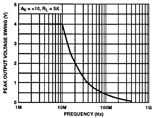
FIGURE 20. OUTPUT VOLTAGE SWING vs FREQUENCY
