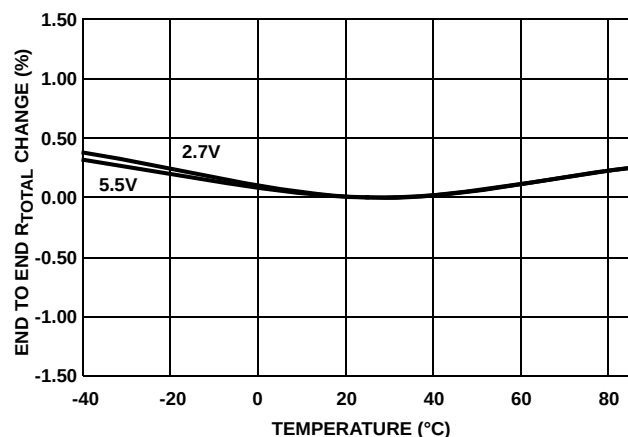
FIGURE 7. END TO END R_{TOTAL} % CHANGE vs TEMPERATURE
