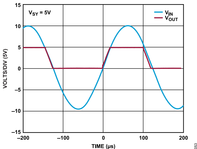
Figure 55. ADA4098-1 and ADA4098-2 as Unity-Gain Buffer with Noninverting Input Driven Beyond the Supply ( V_{SY} = 5\text{ V} )
