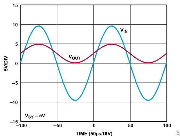
Figure 67. \pm 10 V to 0 V to +5 V Funnel Amplifier, Input and Output Voltages
