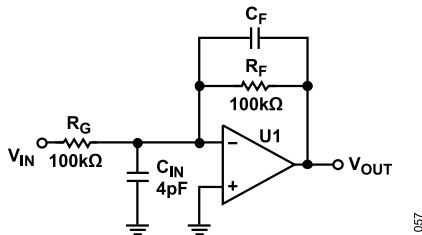
Figure 58. Inverting Gain Schematic
