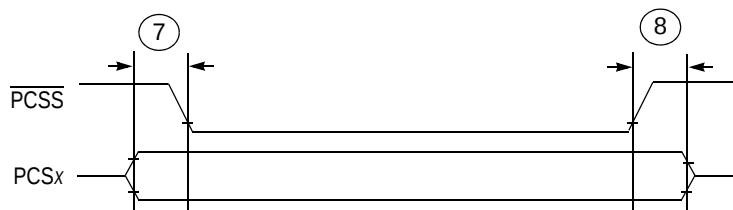
Figure 34. DSPI PCS strobe ( \overline{\text{PCSS}} ) timing
