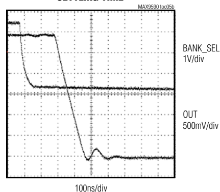
SETTLING TIME
