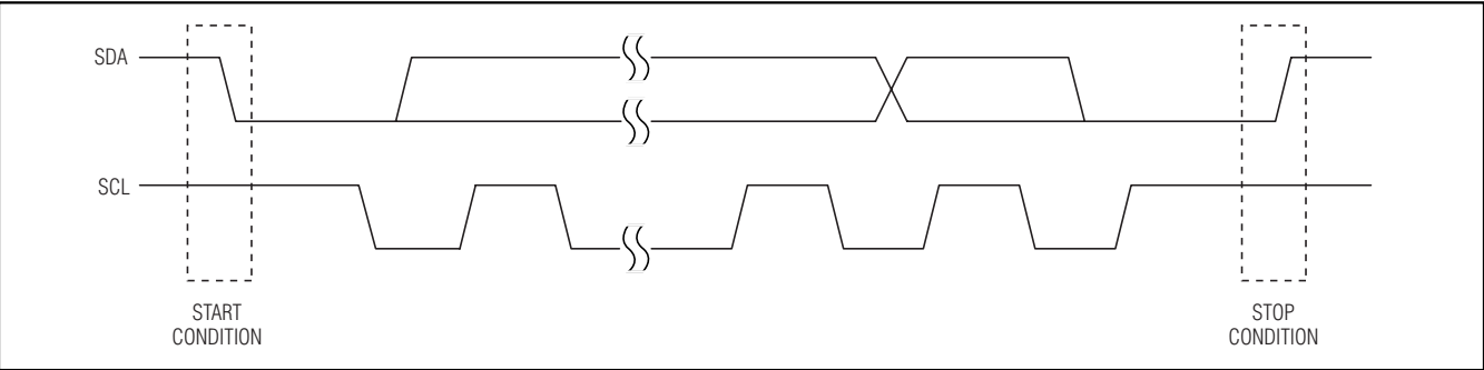
Figure 3. START/STOP Conditions
