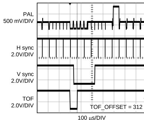
Figure 14. PAL Reference and Output TOF Pulse (TOF_OFFSET = 312)
