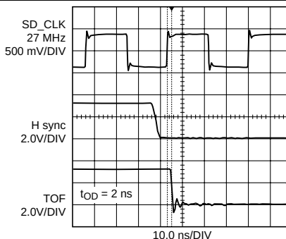
Figure 3. 1080i/50 TOF Pulse
