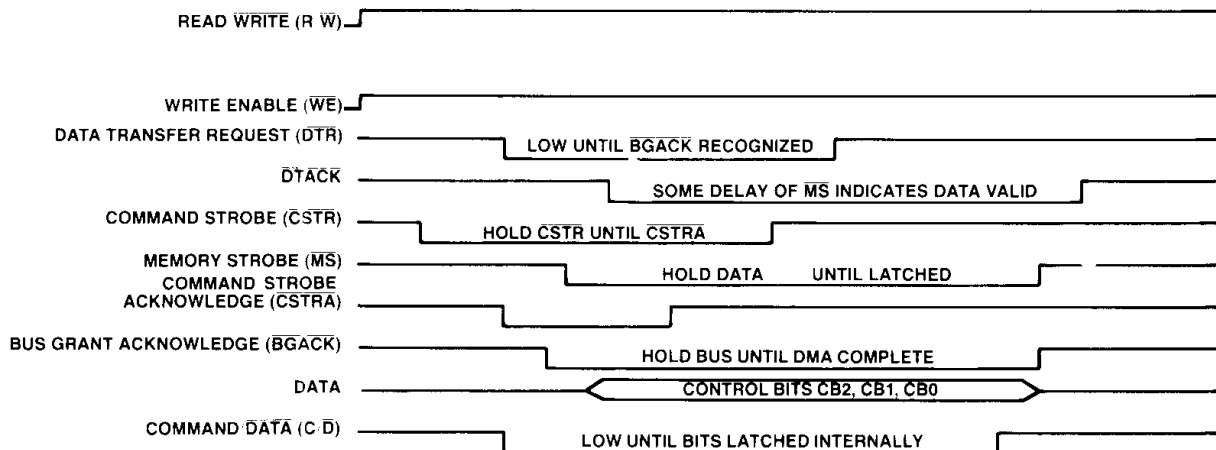
FIGURE 1: BUS CONTROLLER TIMING SEQUENCE
