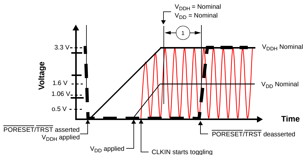
Figure 2-6. Start-Up Sequence with V_{\text{DDH}} Raised Before V_{\text{DD}} with CLKIN Started Before V_{\text{DD}} = 0.5 \text{ V}
