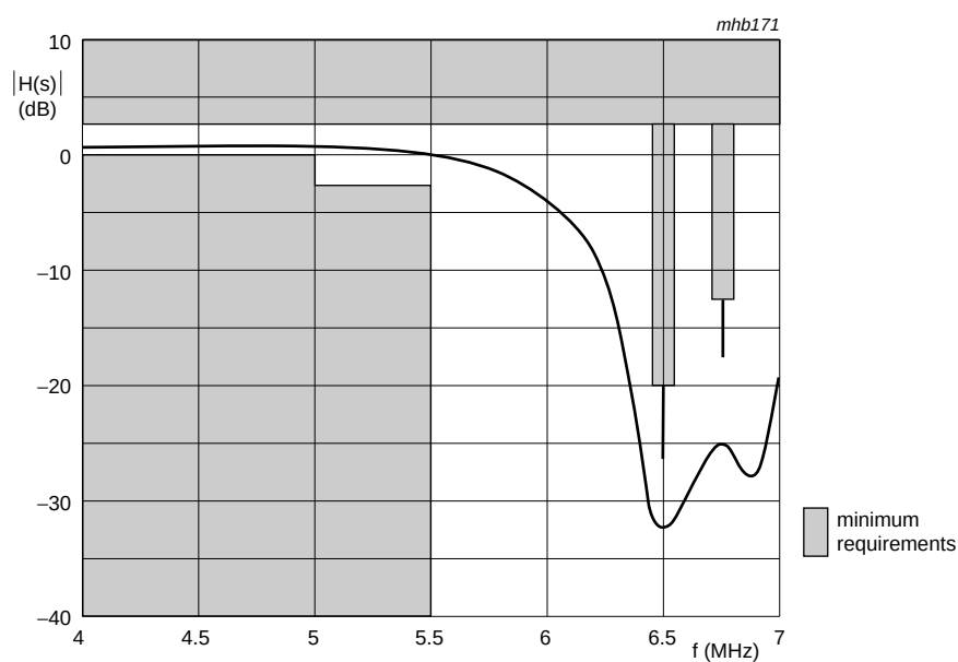
Fig.20 Typical amplitude response for sound trap at D/K standard.
