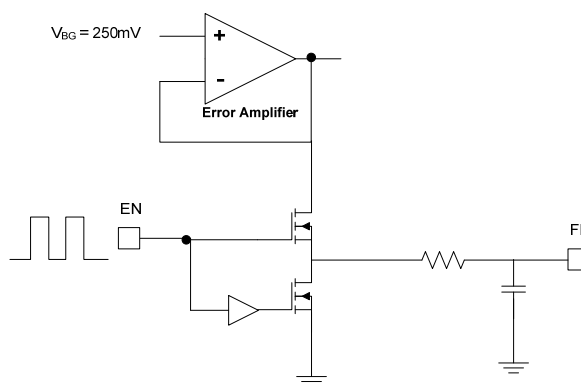
Figure 28. Block Diagram of FB and EN Circuit for PWM Dimming
