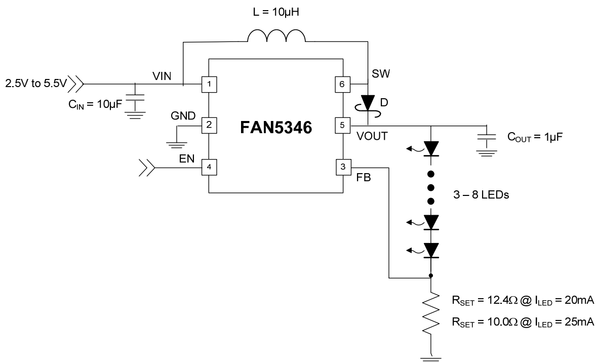
Figure 1. Typical Application
