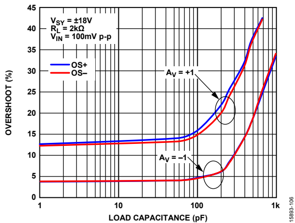
Figure 37. ADA4625-2 OS± vs. Load Capacitance, V_{SY} = \pm 18\text{ V}
