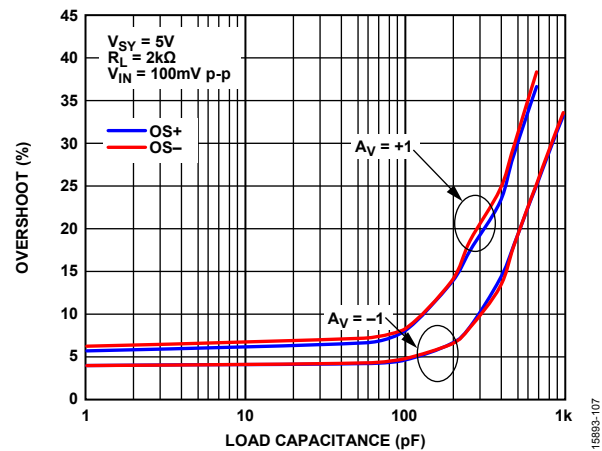
Figure 40. ADA4625-2 OS± vs. Load Capacitance, V_{SY} = 5\text{ V}
