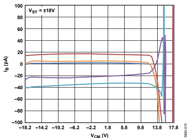
Figure 17. I_B vs. V_{CM} , V_{SY} = \pm 18\text{ V}
