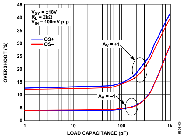
Figure 36. ADA4625-1 Small Signal Overshoot (OS±) vs. Load Capacitance, V_{SY} = \pm 18\text{ V}
