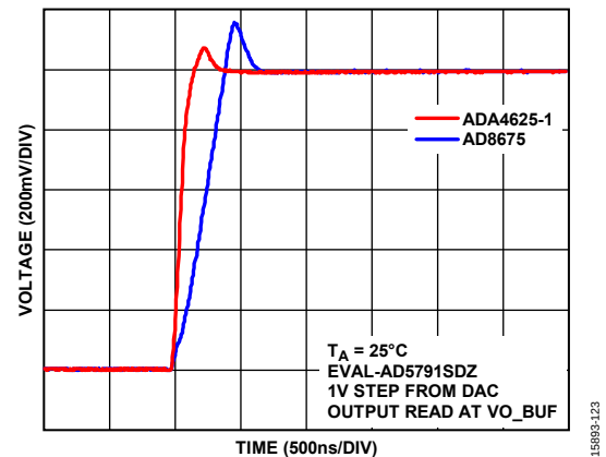
Figure 107. Step Response with ADA4625-1 and AD8675 Output Buffers
