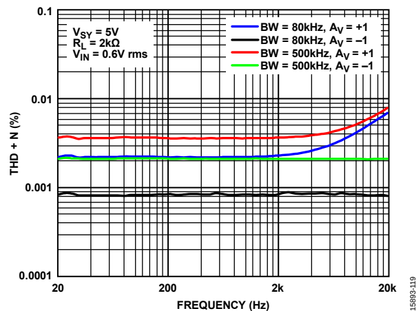
Figure 80. ADA4625-2 THD + N vs. Frequency, V_{SY} = 5V
