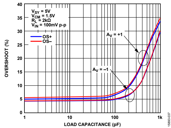
Figure 39. ADA4625-1 OS± vs. Load Capacitance, V_{SY} = 5\text{ V}
