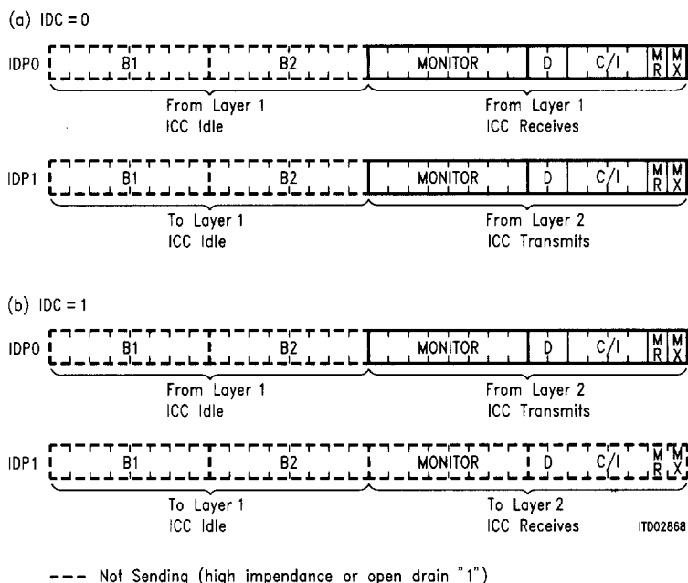
Figure 27 IOM® Data Ports 0, 1 in Non-Terminal Mode (SPM = 1)
