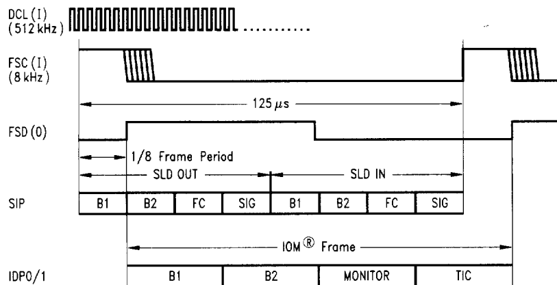
(b) Timing Mode 1
