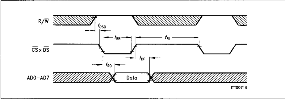
Figure 39 \mu P Read Cycle
