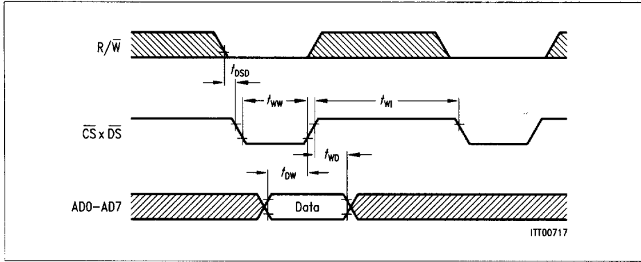
Figure 40 \mu P Write Cycle
