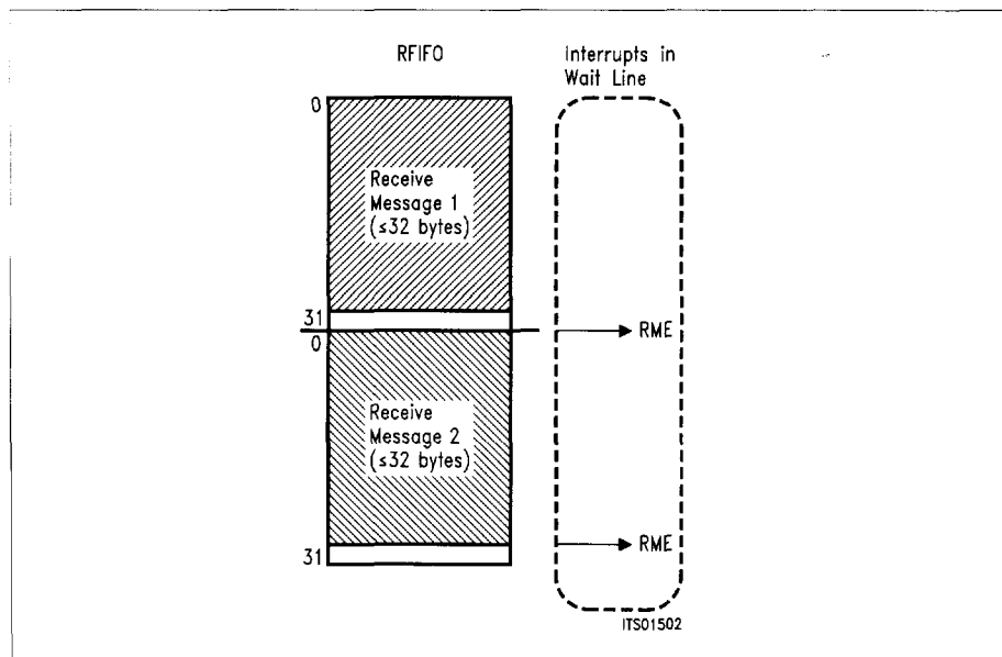
Figure 14 Contents of RFIFO (short message)
