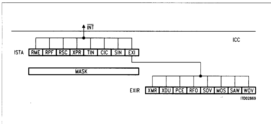
Figure 29 ICC Interrupt Structure
