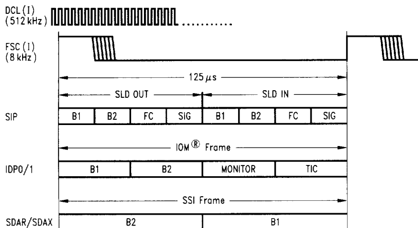
(a) Timing Mode 0
