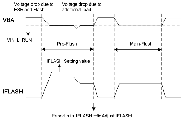
Figure 13: Pre-Flash Operation
