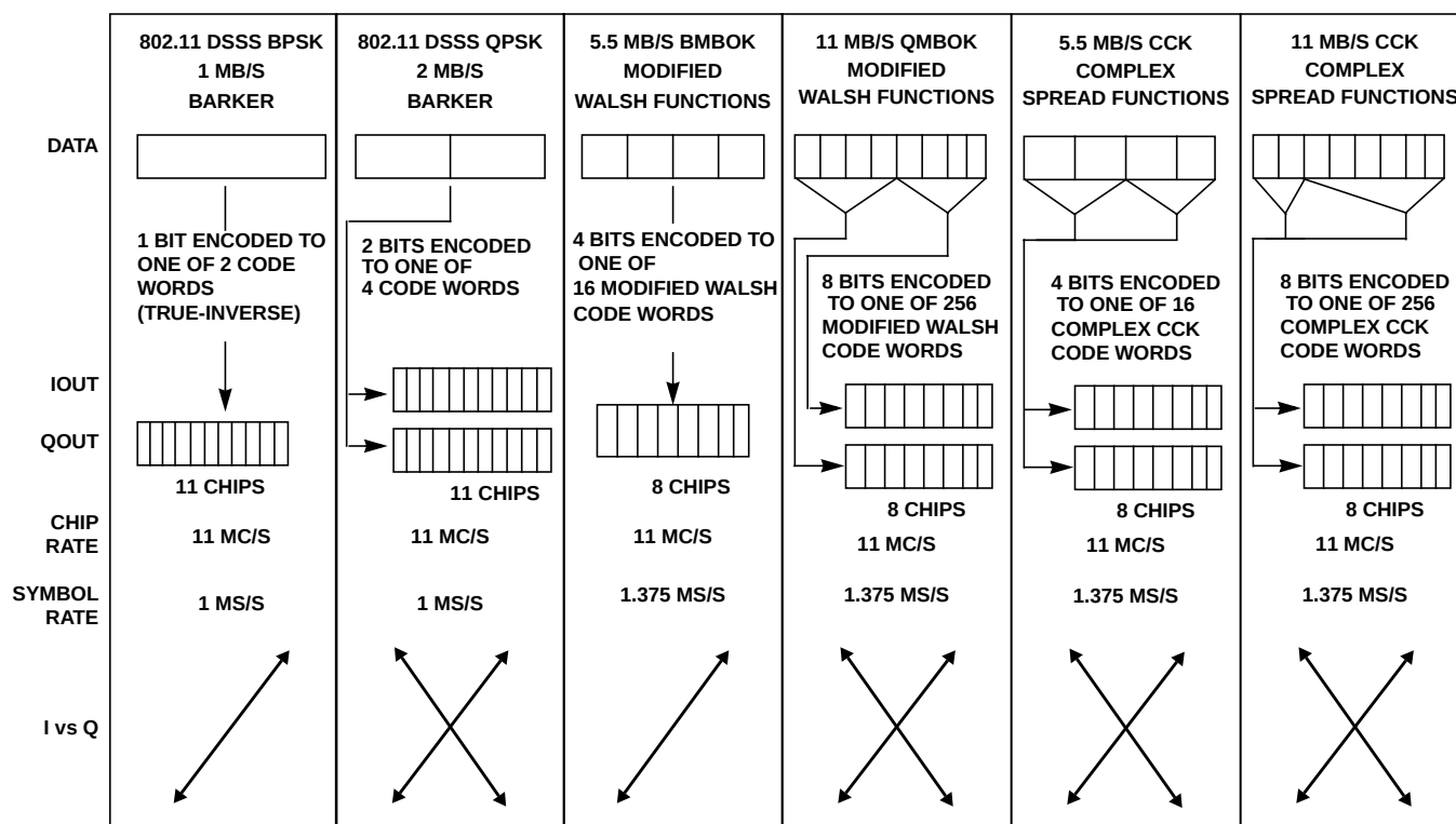
FIGURE 8. MODULATION MODES
