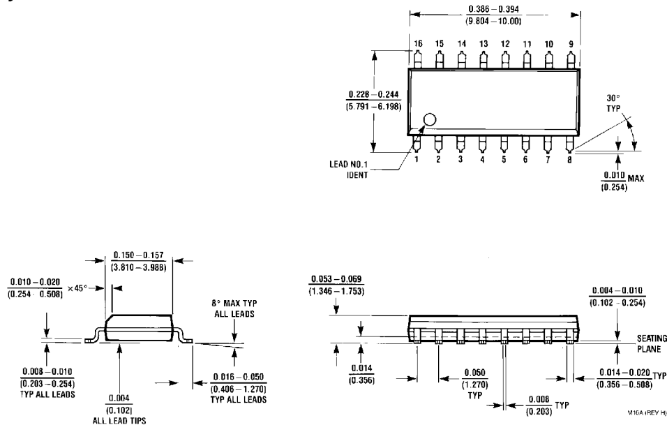
16-Lead Small Outline Molded Package (M) Order Number DM74LS368AM NS Package Number M16A
