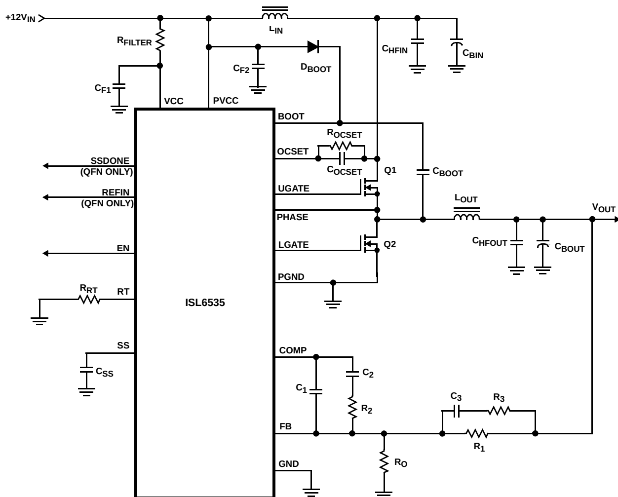
FIGURE 3. TYPICAL APPLICATION
