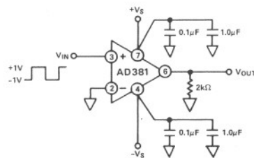
Figure 27a. AD381 Overdrive Recovery Test Circuit
