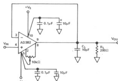
Figure 24a. AD382 Unity Gain Follower
