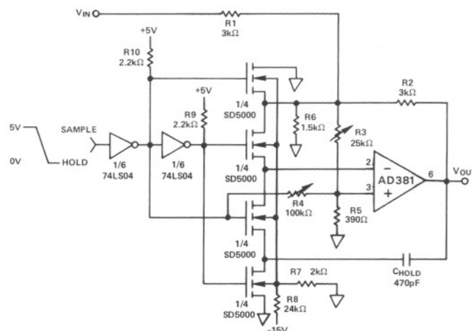
Figure 34. Fast Sample/Hold Amplifier
