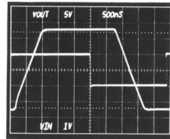
Figure 25b. AD382 Overdrive Recovery Response
