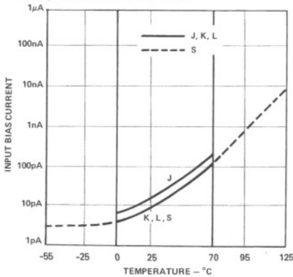
Figure 8. Input Bias Current vs. Temperature
