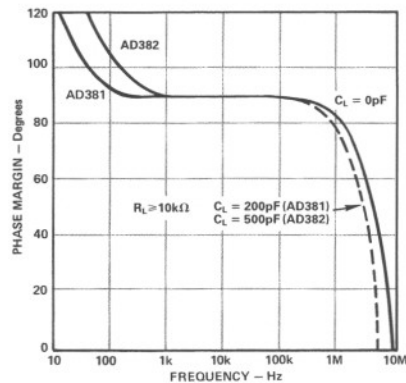
Figure 15. Phase Margin vs. Frequency
