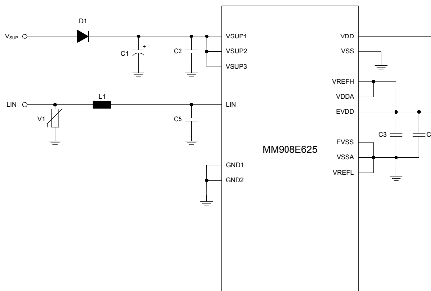
Figure 18. EMC/EMI Recommendations
