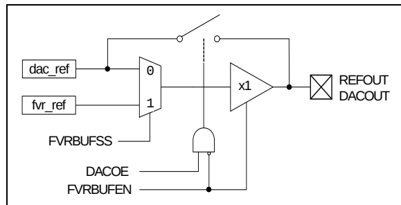
FIGURE 14-3: DAC/FVR OUTPUT PIN
