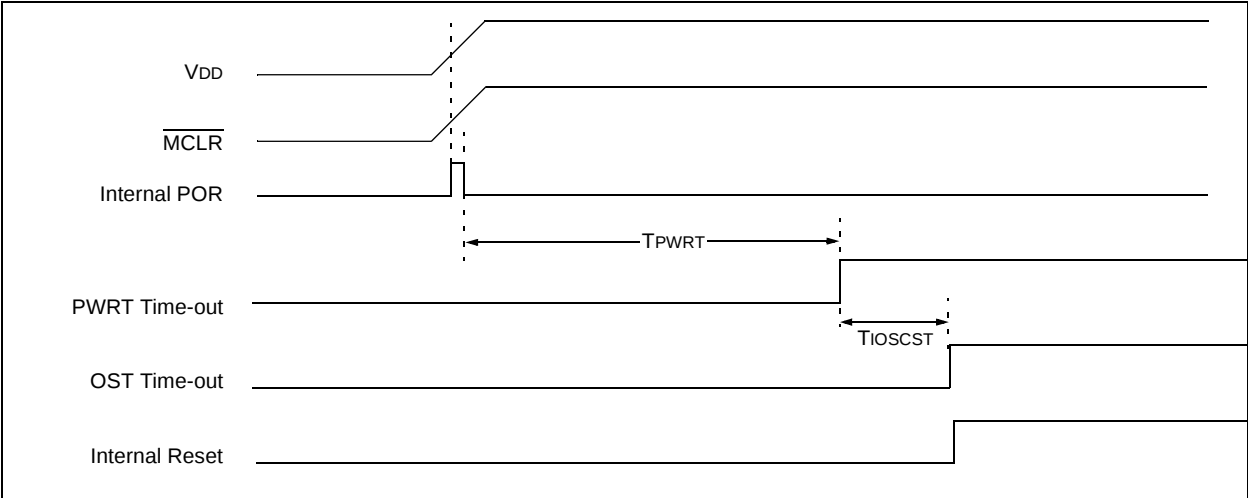
FIGURE 17-6: TIME-OUT SEQUENCE ON POWER-UP (MCLR WITH VDD)
