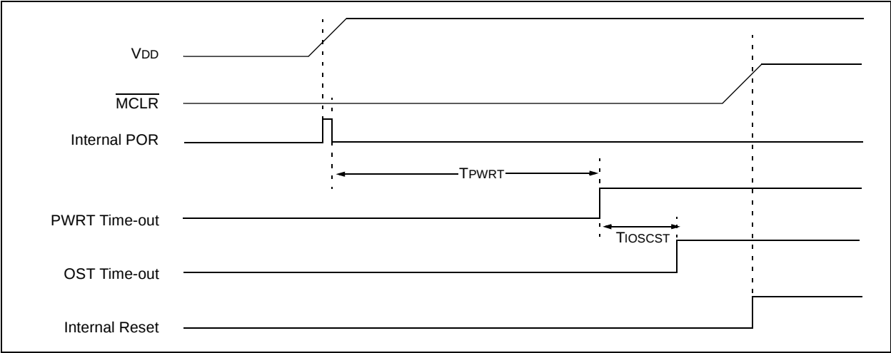
FIGURE 17-5: TIME-OUT SEQUENCE ON POWER-UP (DELAYED MCLR): CASE 2
