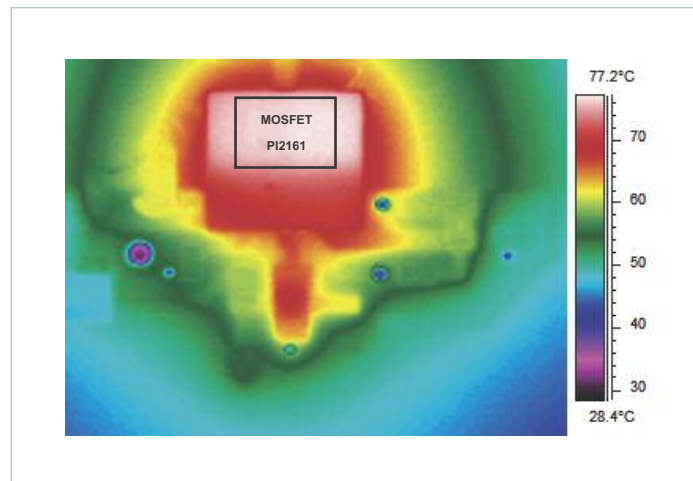
Figure 18 — PI2161 mounted on a 1in² pad of 0.5 oz copper. Thermal Image picture, I_{OUT} = 10 \text{ A} , T_A = 25^\circ\text{C} , Air Flow = 0 LFM
