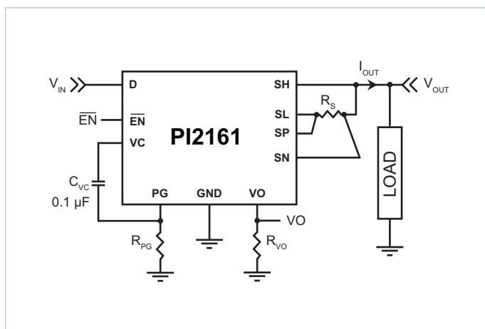
Figure 1 — PI2161 High Side Disconnect switch
