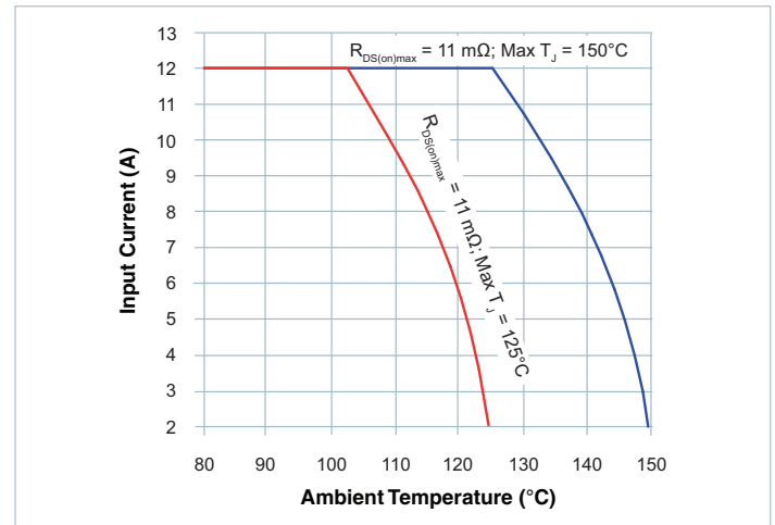
Figure 17 — PI2161 input current de-rating vs. PCB temperature, for the MOSFET maximum T_J at 125°C and 150°C
