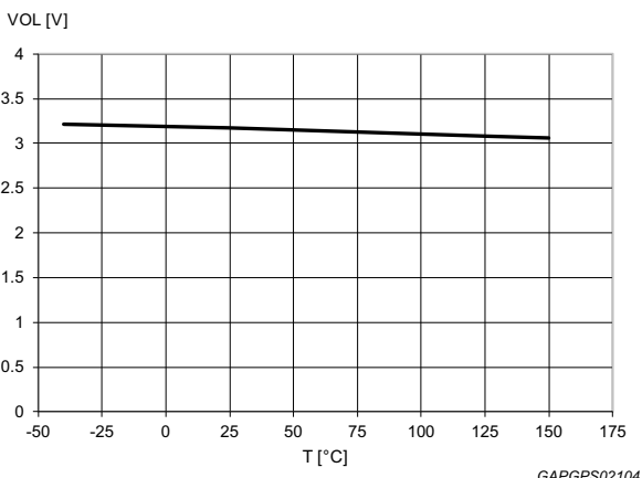
Figure 32. OFF-state open-load voltage detection threshold
