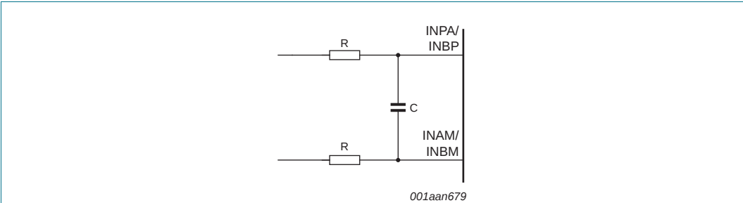
Fig 7. Anti-kickback circuit
