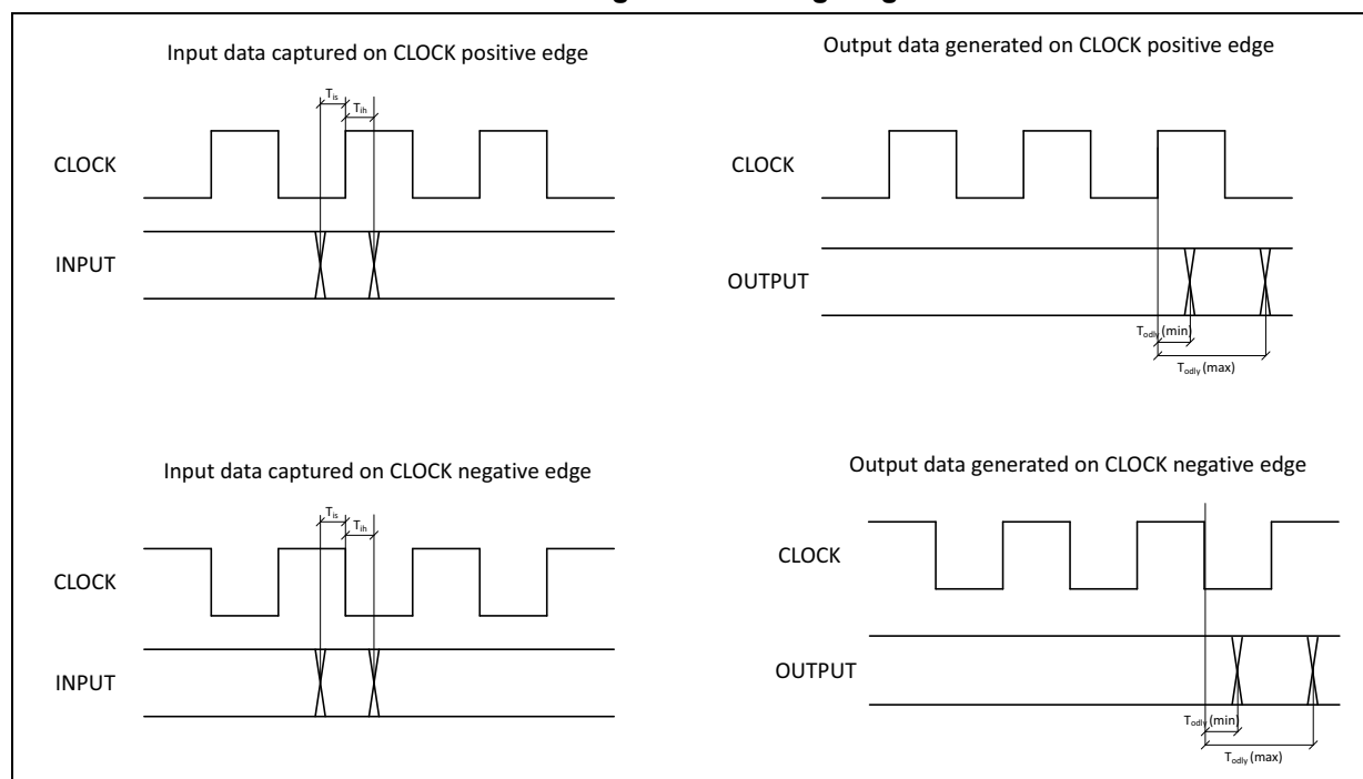
Figure 13. Timing diagrams
