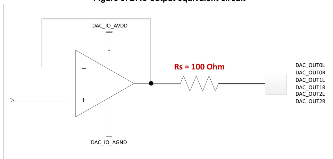
Figure 9. DAC output equivalent circuit
