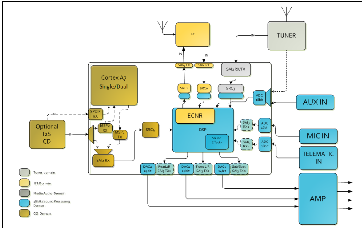
Figure 2. Accordo5 sound subsystem application example
