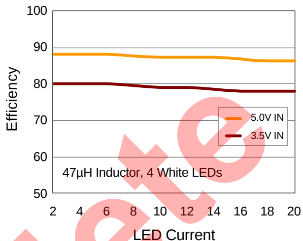
LX1995-2 EFFICIENCY
