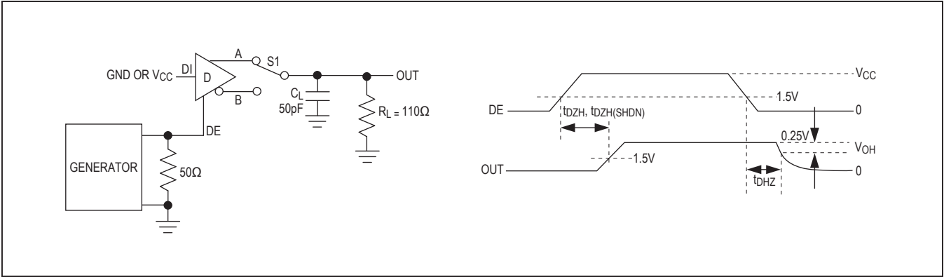
Figure 4. Driver Enable and Disable Times ( t_{DHZ} , t_{DZH} )
