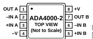
Figure 4. 8-Lead MSOP (RM-8)
