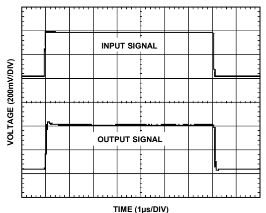
Figure 32. Capacitive Load with Snubber Network
