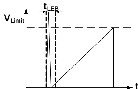
Figure 4: Leading-Edge Blanking
