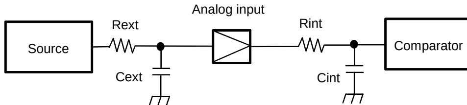
Analogue input circuit model
