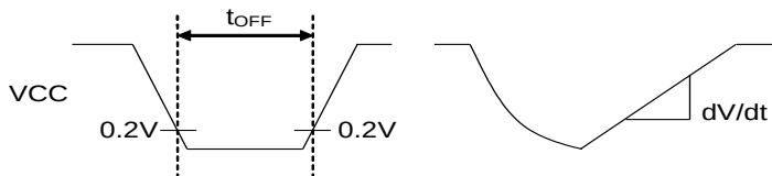
Power off time, Power ramp rate at Power-on
