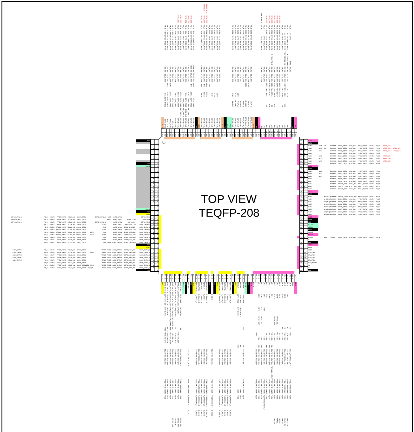
Figure 4-14: TEQFP-208 (S6J323CKxx)
