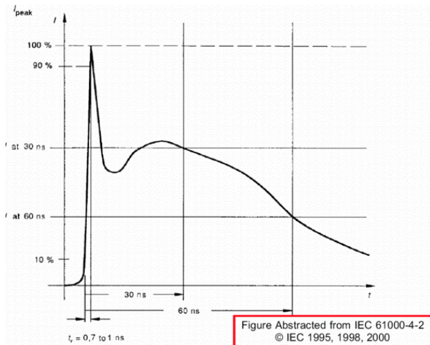
Figure 7. I_{peak} = f(t)/IEC61000-4-2
