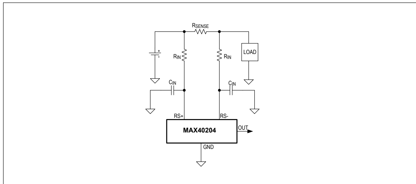
Figure 4. Input Common-Mode Filtering
