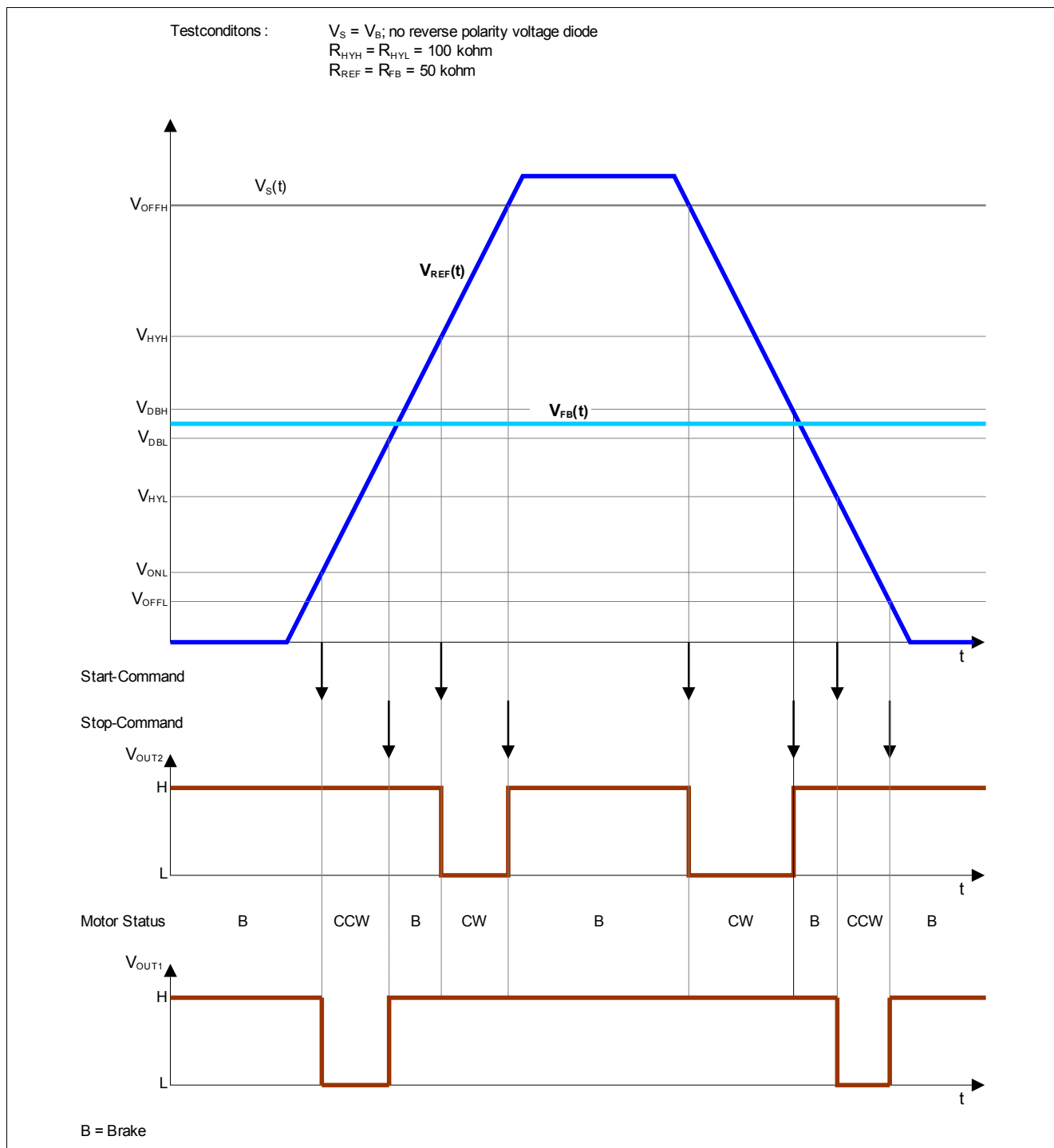
Figure 5 Motor Operation
