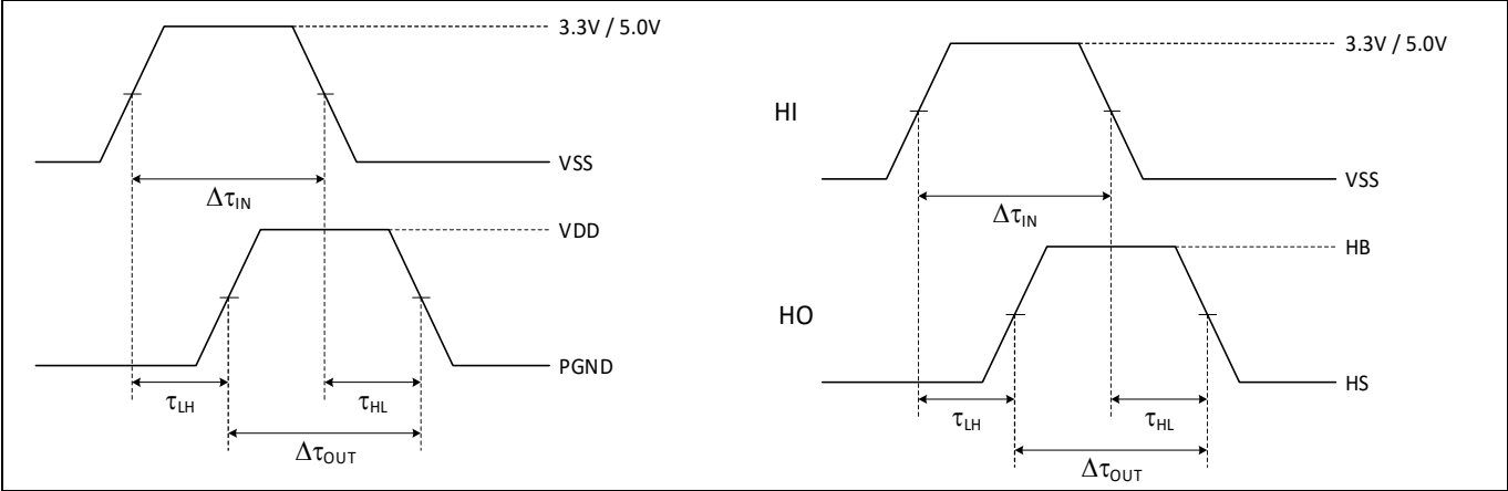
Figure 6 Propagation delay
