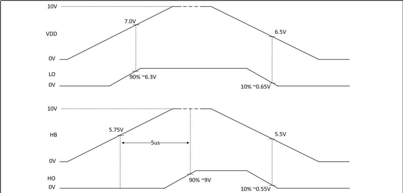
Figure 7 UVLO behavior
