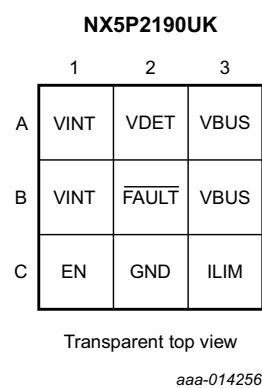
Fig 4. Ball mapping for WLCSP9
