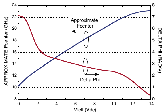
Phase Sensitivity vs. V fctl
