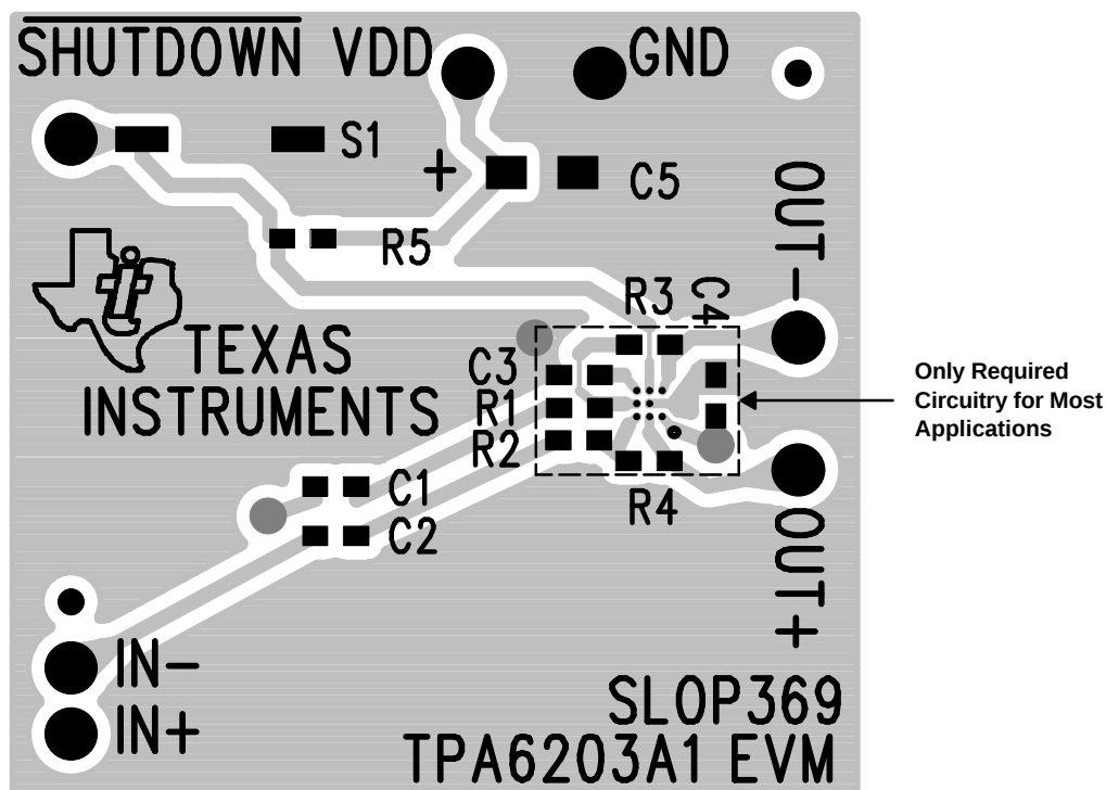
Figure 35. TPA6203A1 EVM Top Layer (Not to scale)
