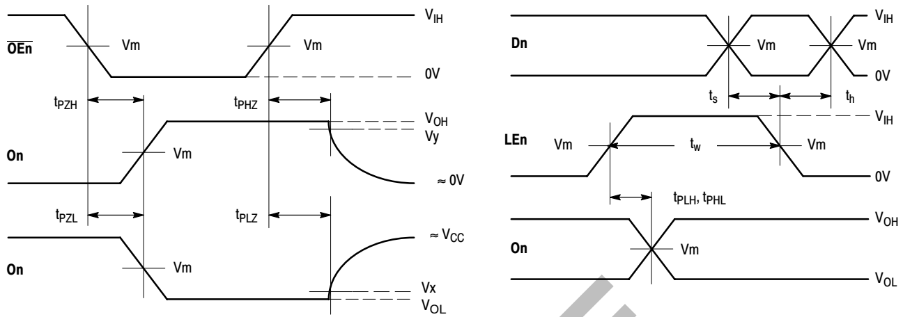
Figure 5. AC Waveforms
