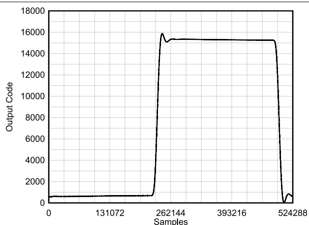
Figure 6-14. Pulse Response
