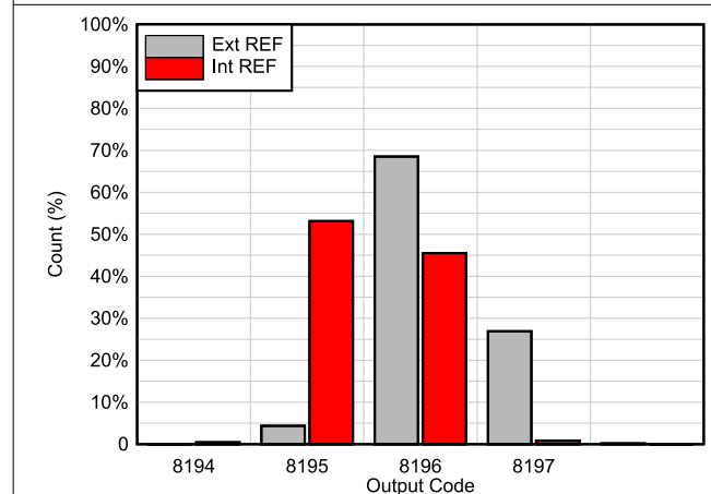
Figure 6-34. DC Histogram
