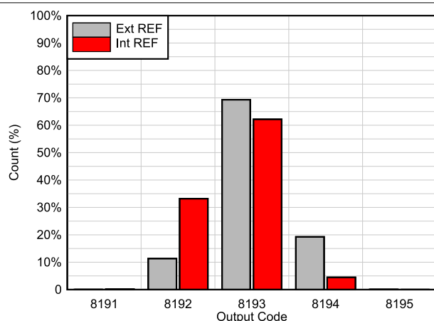
Figure 6-13. DC Histogram
