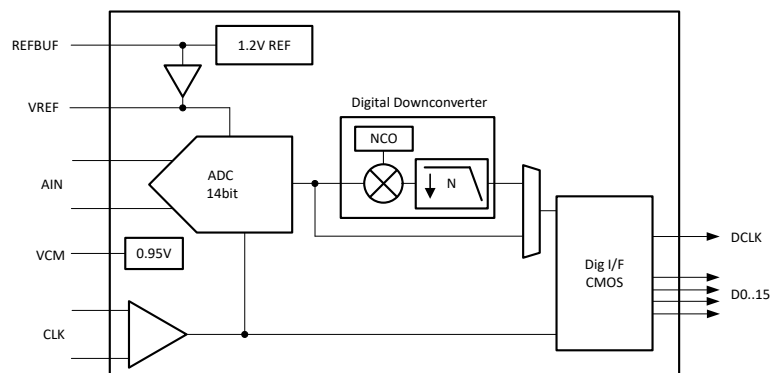
ADC354x Block Diagram
