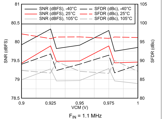
Figure 6-10. AC Performance vs VCM vs Temperature
