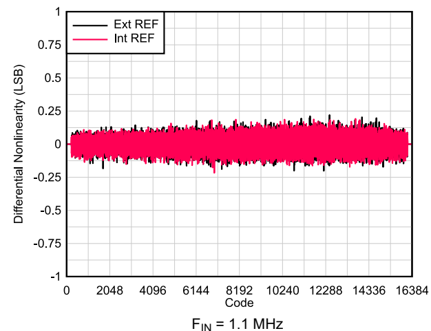
Figure 6-33. DNL vs Code
