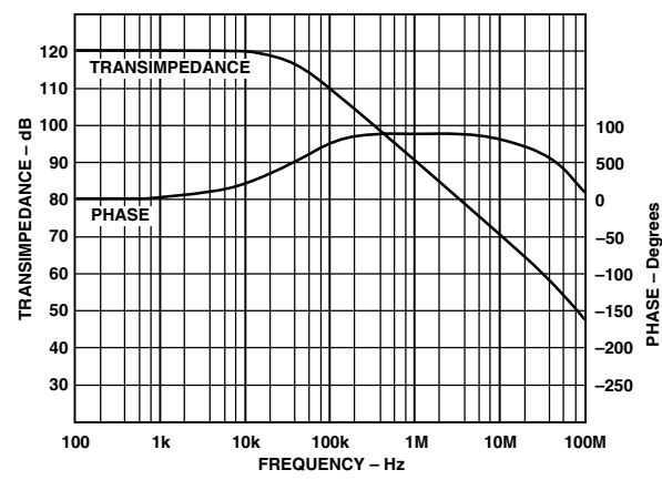
Figure 19. Open-Loop Transimpedance vs. Frequency
