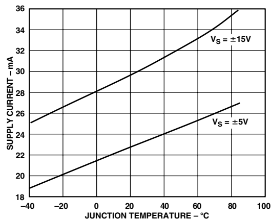
Figure 7. Total Supply Current vs. Temperature
