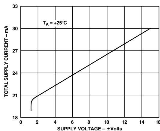
Figure 8. Total Supply Current vs. Supply Voltage
