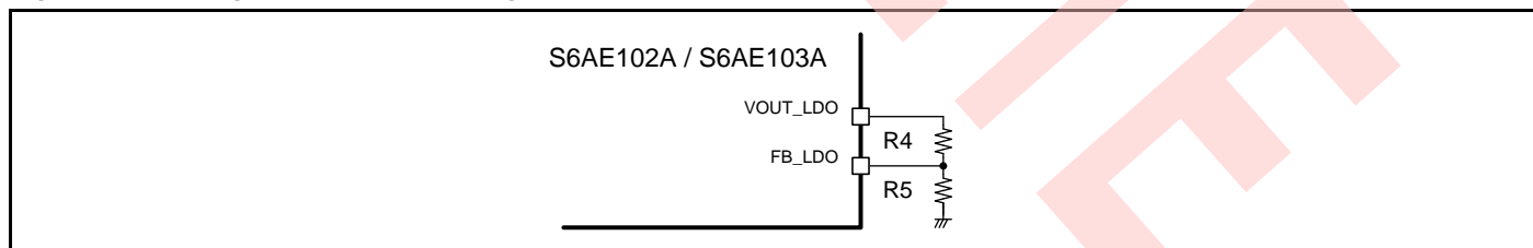
Figure 11-2 Setting of LDO Output Voltage (VOUT_LDO)
