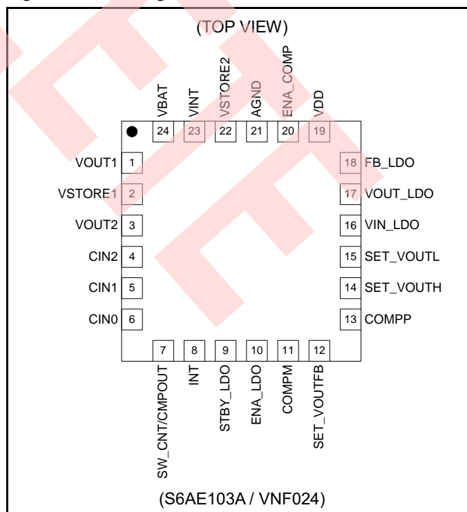
Figure 3-2 Pin Assignment of S6AE103A
