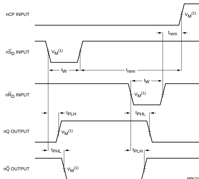
Fig.7 Waveforms showing the set ( \overline{nS_D} ) and reset ( \overline{nR_D} ) input to output (nQ, nQ) propagation delays, the set and reset pulse widths and the \overline{nR_D} , \overline{nS_D} to nCP removal time.
