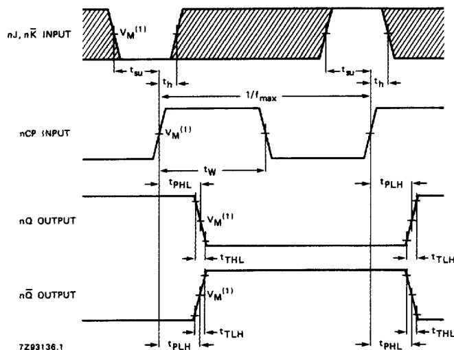
Fig.6 Waveforms showing the clock (nCP) to output (nQ, nQ) propagation delays, the clock pulse width, the nJ, nK to nCP set-up, the nCP to nJ, nK hold times, the output transition times and the maximum clock pulse frequency.
