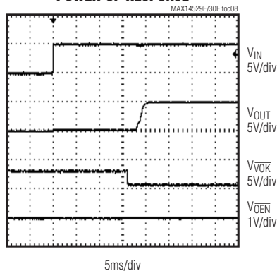
POWER-UP RESPONSE
