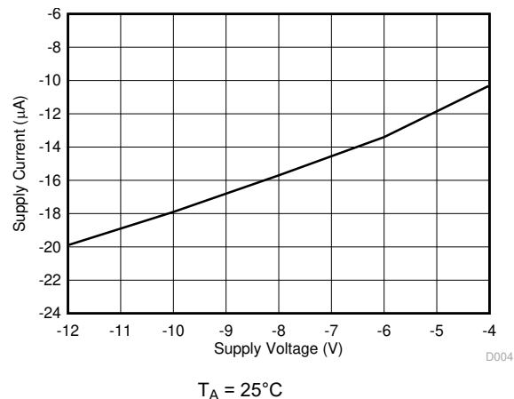
Figure 6-4. Supply Current vs Supply Voltage
