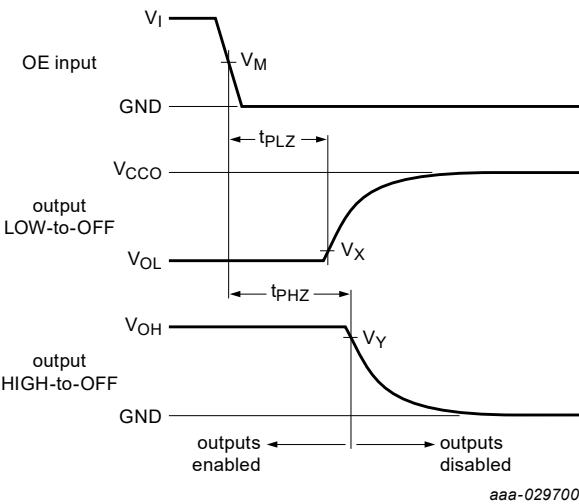
Measurement points are given in Table 14 . V_{OL} and V_{OH} are typical output voltage levels that occur with the output load. V_{CCO} is the supply voltage associated with the output.
