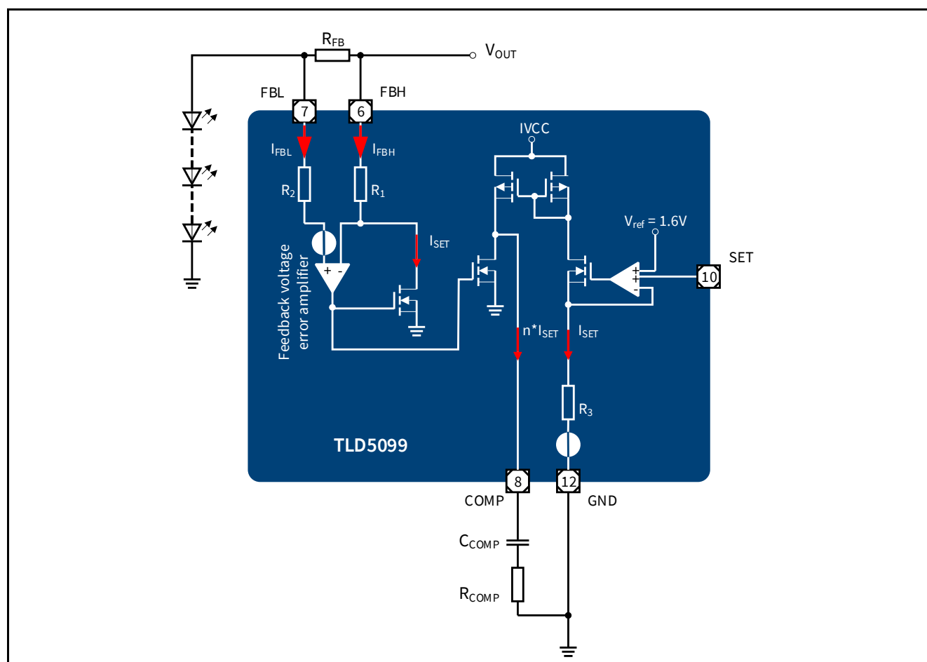
Figure 24 Concept drawing analog dimming
