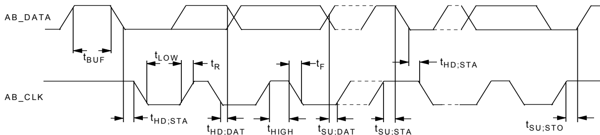
Figure 29.10 I²C/SMBus Timing
