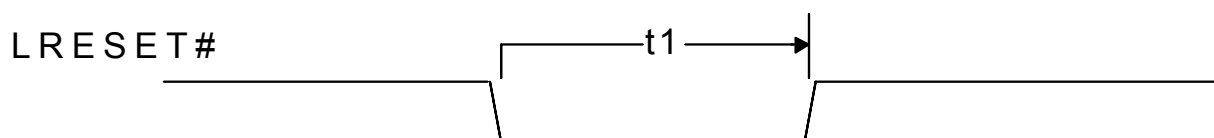
Figure 29.3 Reset Timing
