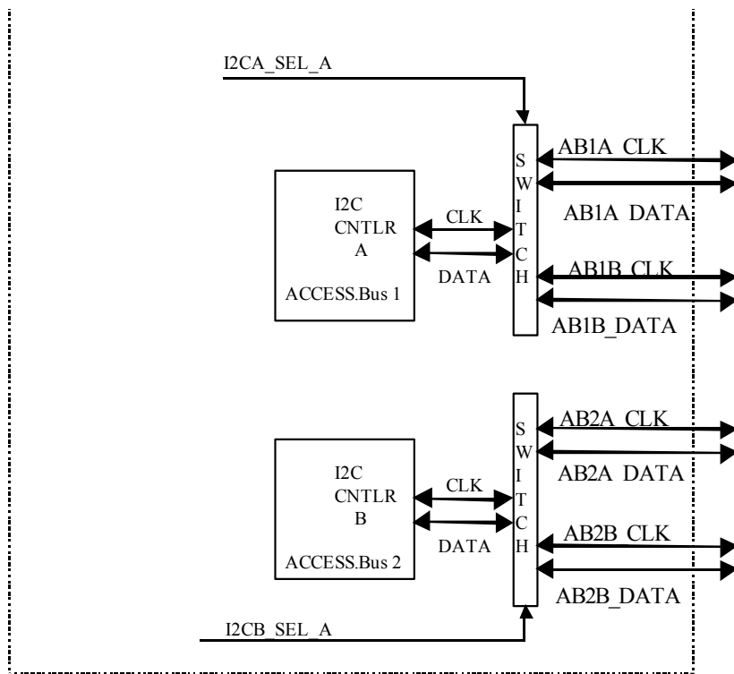
Figure 15.1 I²C/SMBus Controllers
