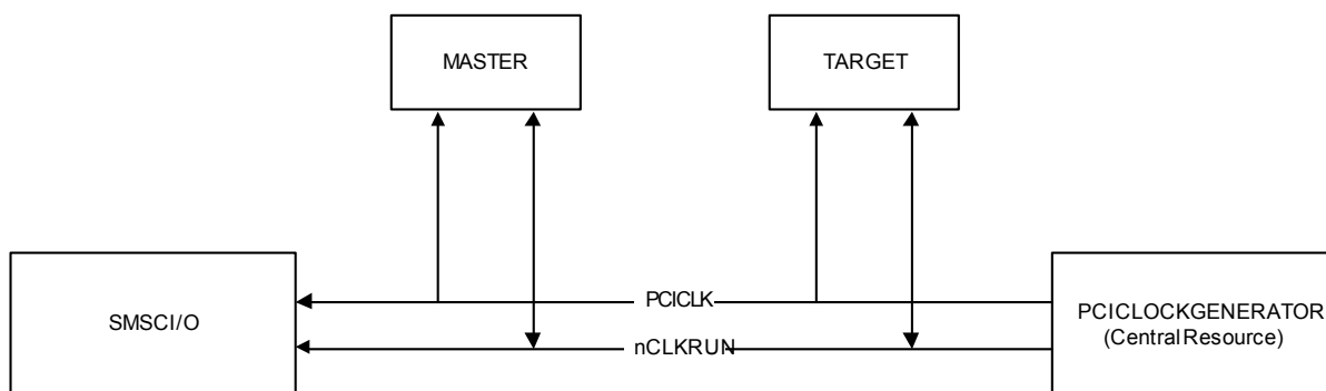
Figure 24.1 CLKRUN# System Implementation Example
