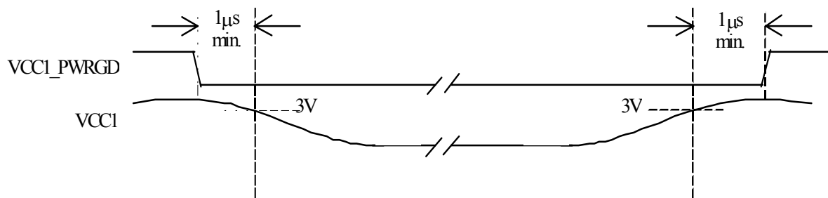
Figure 2.3 VCC1_PWRGD Timing
