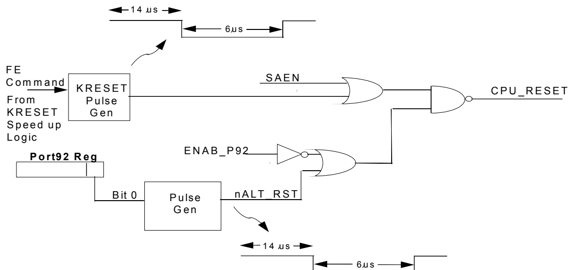
Figure 13.2 CPU_Reset Implementation Diagram
