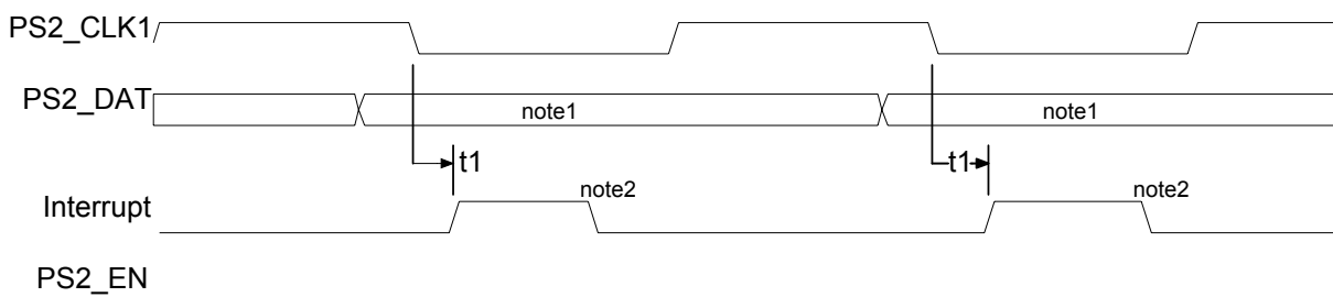
Figure 29.16 PS/2 Channel “Bit-Bang” Receive Timing Diagram
