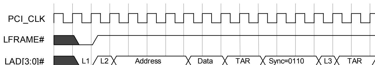
Figure 29.6 I/O Write
