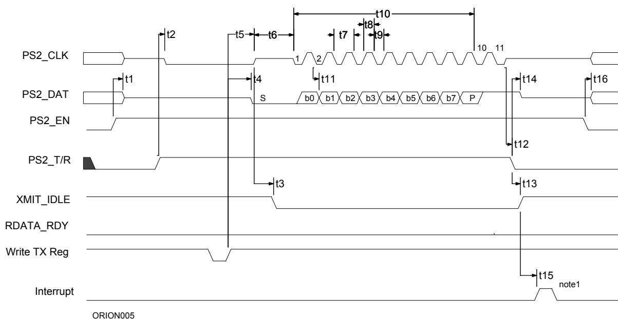
Figure 29.14 PS/2 Channel Transmit Timing Diagram
