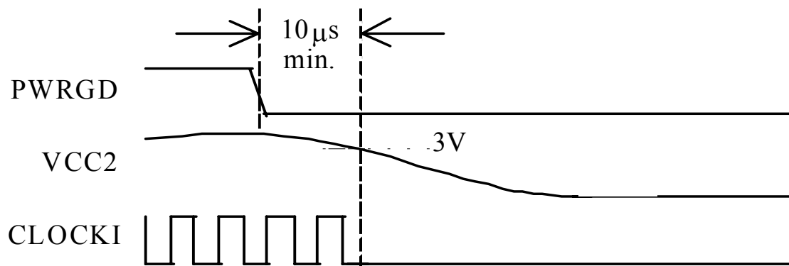
Figure 2.1 Power-Fail Event
