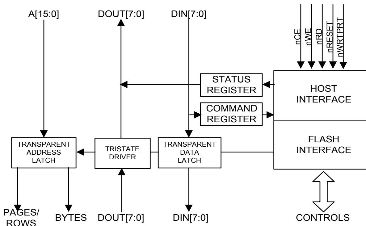
Figure 8.2 CSI Block Diagram
