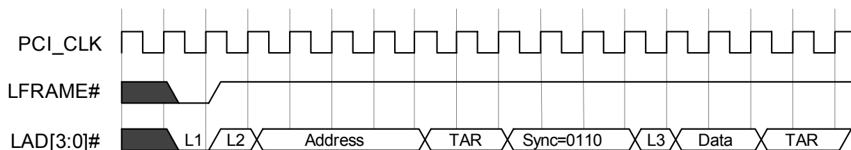
Figure 29.7 I/O Read
