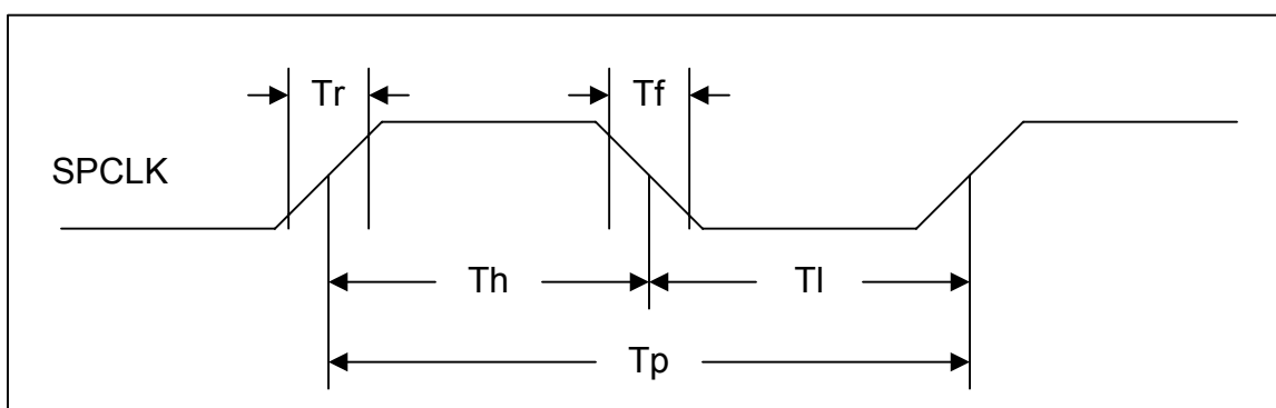
Figure 29.17 SPI Clock Timing
