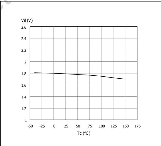
Figure 17. Input low-level
