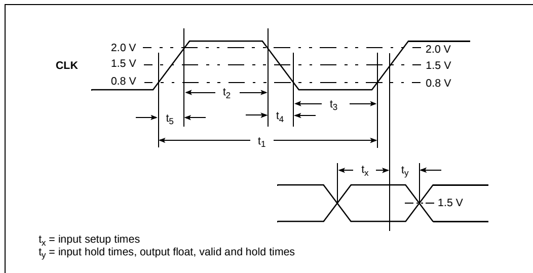
Figure 3. CLK Waveform
