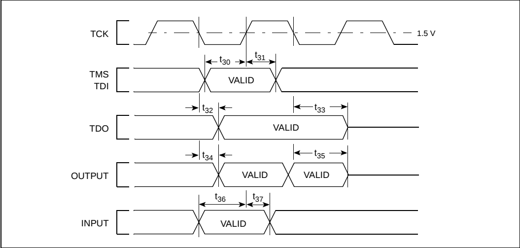
Figure 10. Test Signal Timing Diagram
