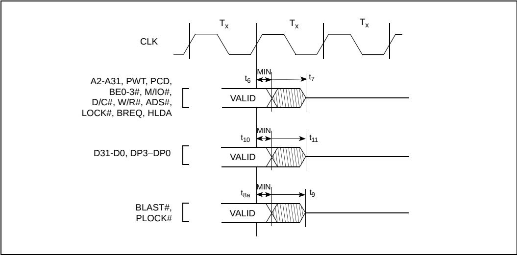
Figure 9. TCK Waveform
