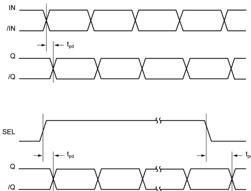
Figure 1. Propagation Delay
