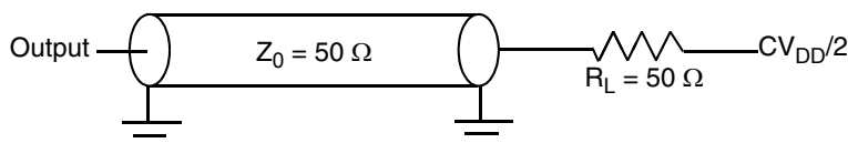
Figure 9. eSPI AC Test Load
