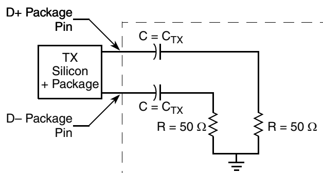
Figure 42. SGMII AC Test/Measurement Load
