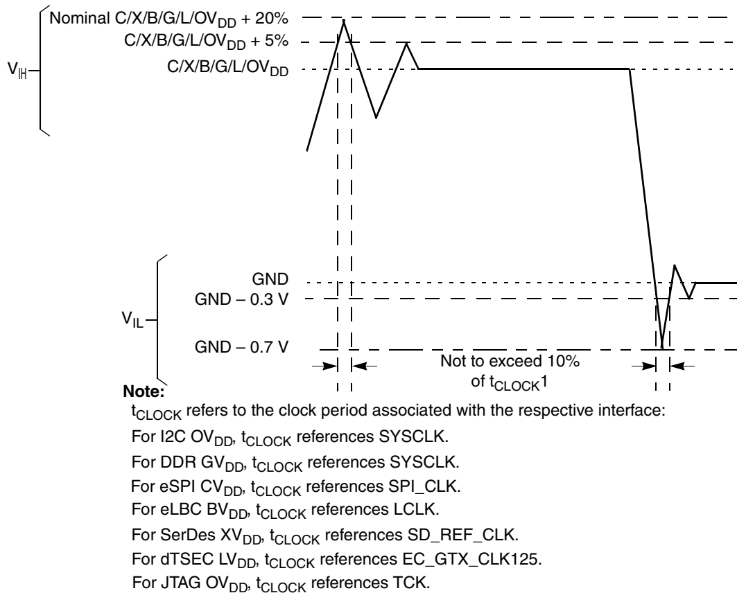
Figure 2. Overshoot/Undershoot Voltage for BV_{DD}/GV_{DD}/LV_{DD}/OV_{DD}/XV_{DD}/CV_{DD}
