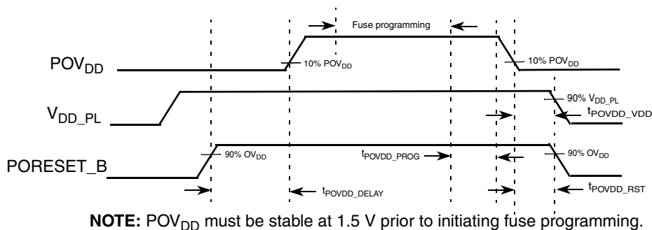
Figure 3. POV_{DD} Timing Diagram
