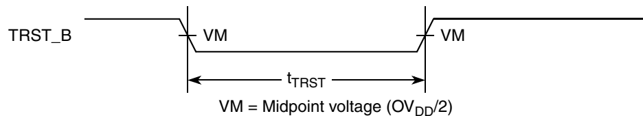
Figure 24. TRST_B Timing Diagram
