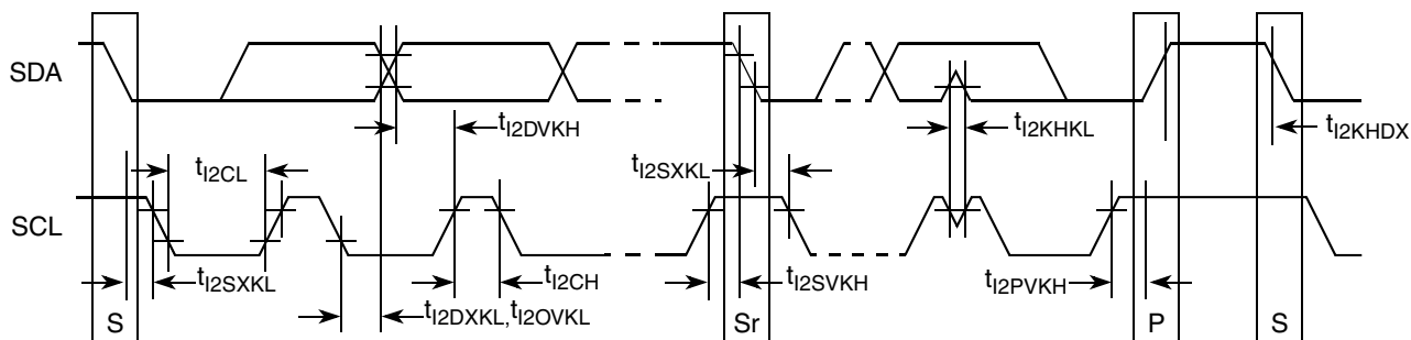
Figure 27. I 2 C Bus AC Timing Diagram
